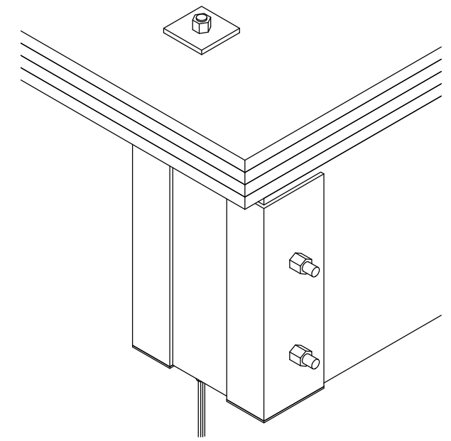
ISOMETRIC W/ GIRDER SUPPORT BOLT SCALE 1:10
